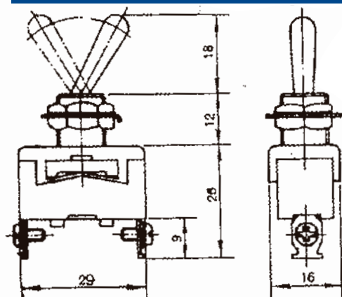
0608591 - On/Off
