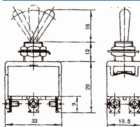
0608592 - On/Off/On
